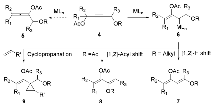
Scheme 2. Controlled [1,2]-acyl shift to form vinyl carbenoid and its trapping.
