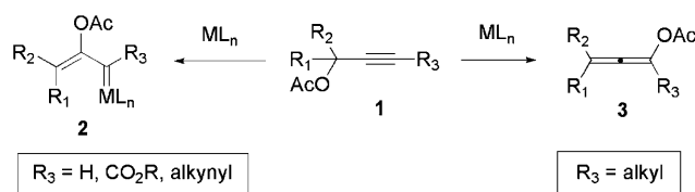
Scheme 1. [1,2]- vs. [1,3]-acyl shift.
