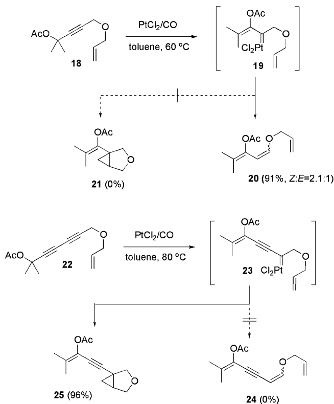
Scheme 4. The reactivity difference between vinyl and alkynyl Pt-carbenoids.
