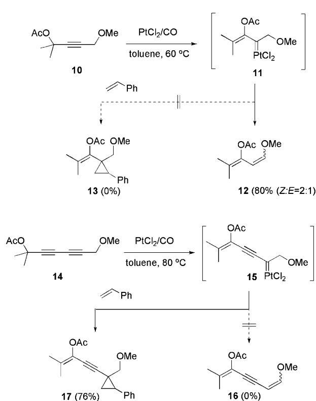
Scheme 3. The reactivity difference between vinyl and alkynyl Pt-carbenoids.
